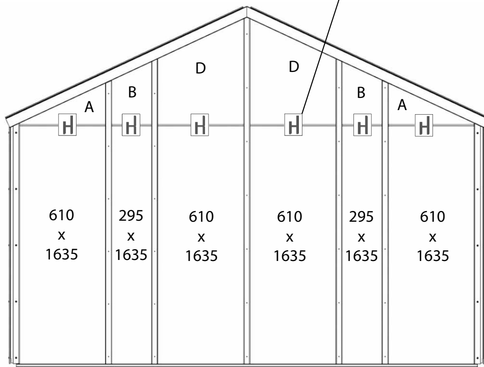
Rear End
