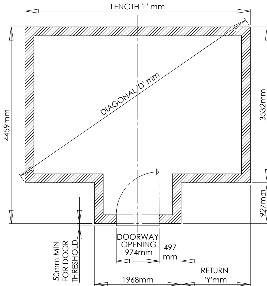
DIMENSION VARIABLES (mm)
