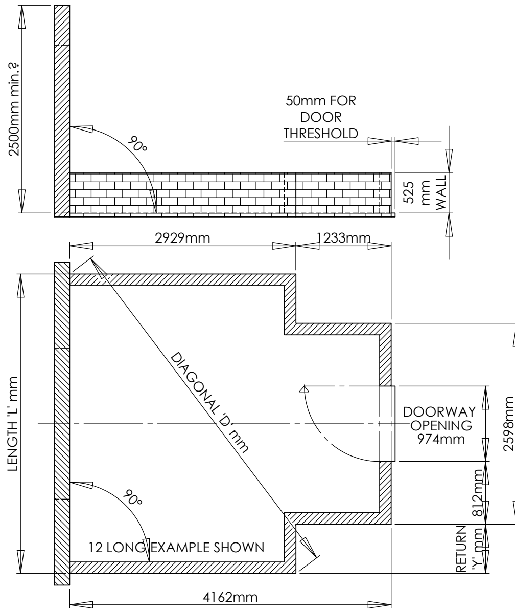
DIMENSION VARIABLES (mm)
